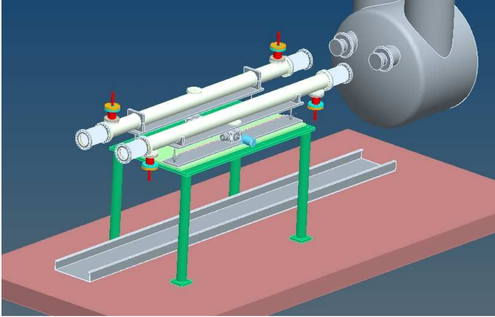
Figure 9: View of two long-range beam-beam compensators in the RHIC ring, mounted on a vertically movable stand. To the right the triplet cryostat is visible, under the beam pipes is a cable tray (courtesy of R. Alforque).
