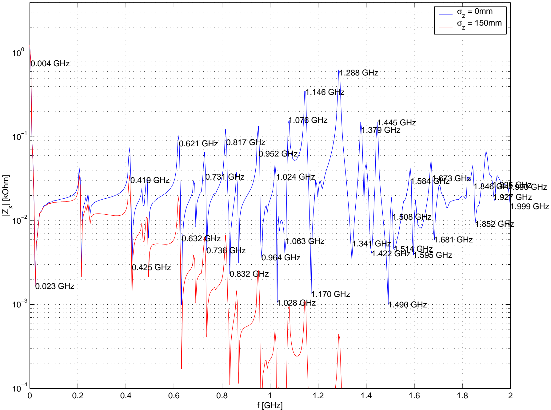
Impedance and Wake of BBLR for dx=dy=dz=2\text{mm}
