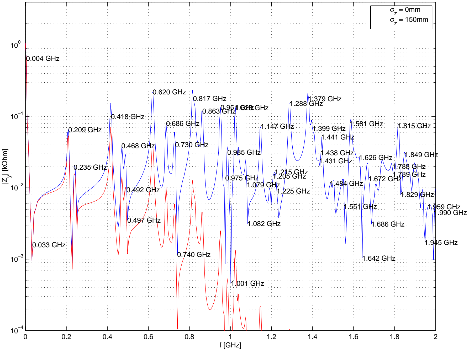
Impedance and Wake of BBLR for dx=dy=dz=2mm
