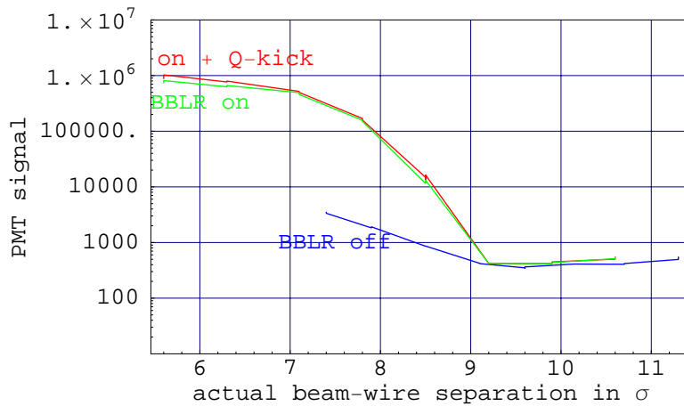
Figure 3: PMT losses versus beam-wire separation
