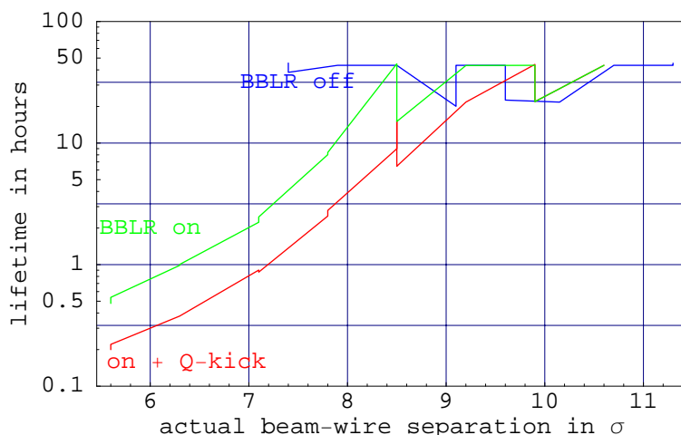
Figure 4: Current losses versus beam-wire separation
