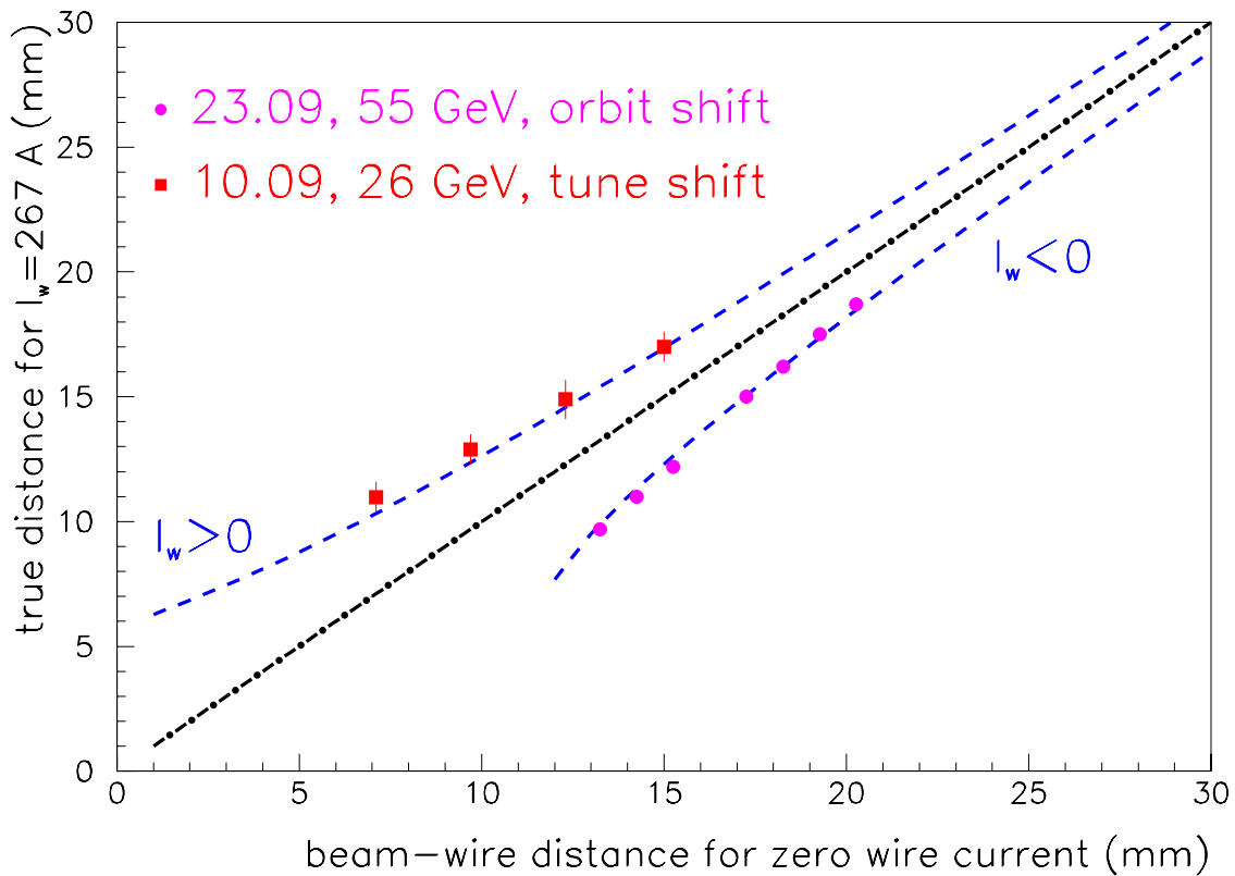
Figure 2: The actual distance between wire and beam for I_w = 267 A as a function of the same distance without wire excitation. The dashed line is the theoretical prediction (see MD note 2), the upper plotting symbols refer to the four tune shift measurements after 17:30 in MD2 at 26 GeV; the lower symbols refer to the local orbit shift measured in the present MD after 5:46 at 55 GeV/c. Note that for the 1st MD the first point (15.0 mm on the horizontal axis) was chosen as a reference and set to the predicted value of 17.0 mm. For the 2nd MD all numbers are measured.
