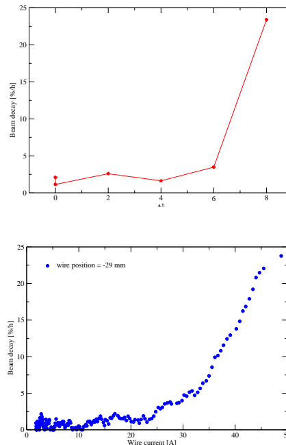
Figure 4: Yellow beam loss rate as a function of vertical chromaticity change (top) with the wire at fixed position -29 mm, and Yellow beam loss rate as a function of wire current at the maximum chromaticity setting (bottom). For the data in the latter plot the wire current was gradually turned off.
