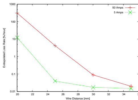
Figure 8: Loss rate as a function of wire distance for 5 A and 50 A wire current, calculated with PLIBB, for the Blue beam in experiment 2 [8].
