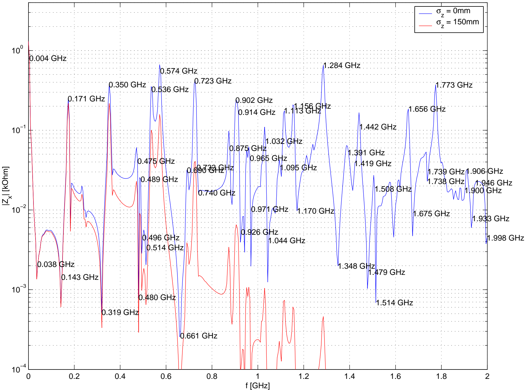
Impedance and Wake of BBLR for RES B BLR S C d xyz2mm s 50m/scratch.
