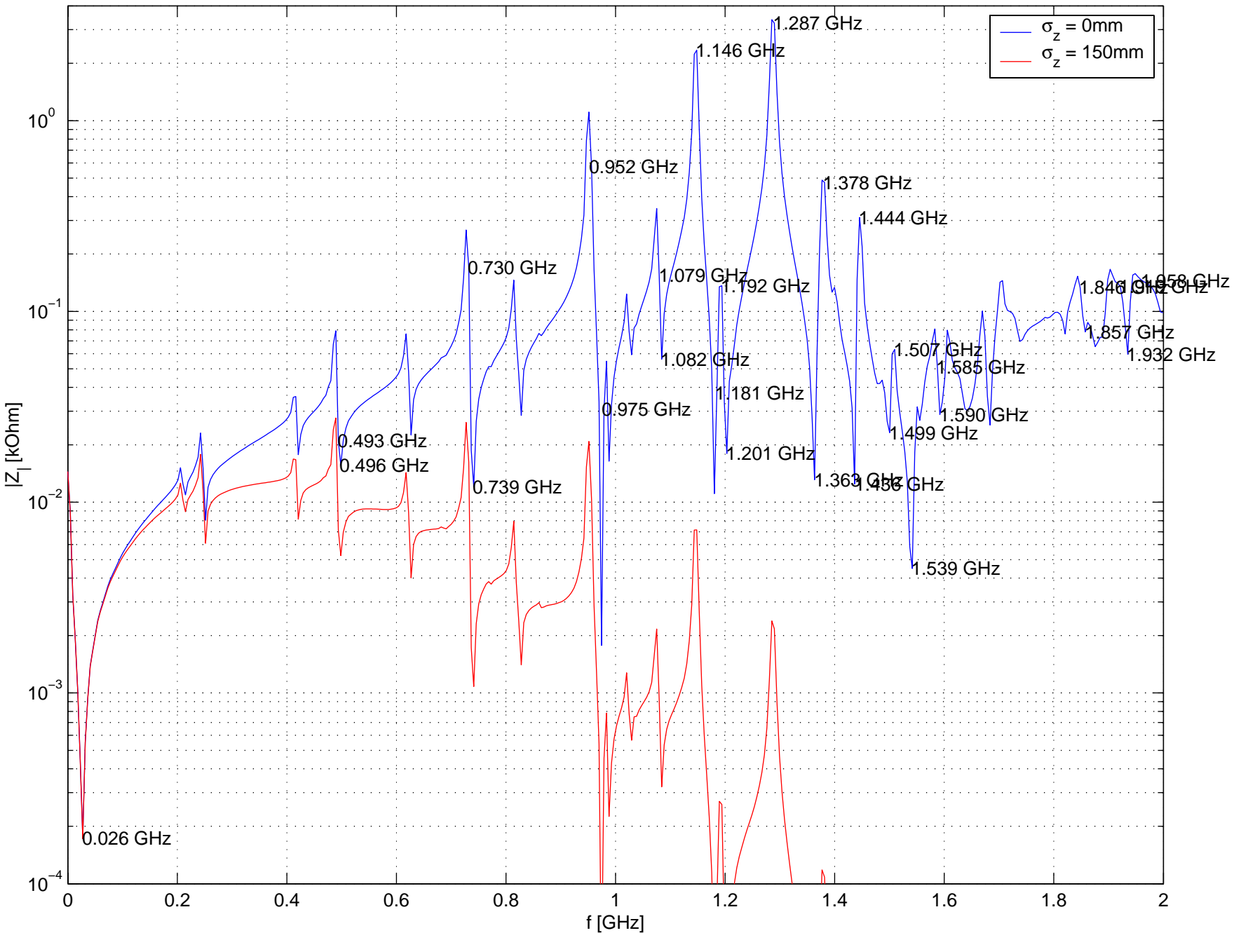
Impedance and Wake of BBLR for dx=dy=dz=2\text{mm}
